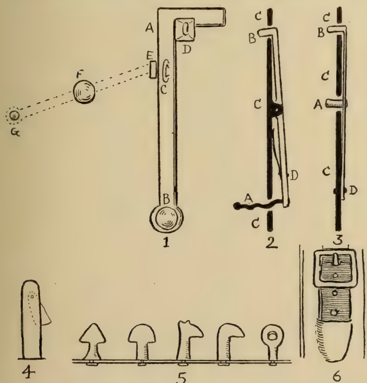
FIG. 33. Locking hooks, turning pins, and strap-cover.
