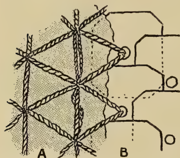
FIG. 25. Construction of Jack. A. Outside. B. Plates with cover and cords removed.
